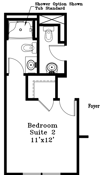
Powder + Private Bath @ Bedroom 2 Suite (4' Extension Recommended - 4' Shown ~ 11'x9' Bedroom w/2' extension)
