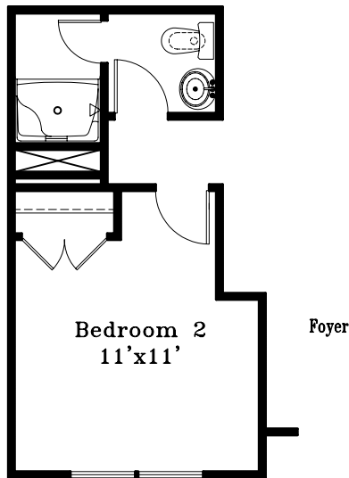
Bedroom 2 with Optional Hybrid Bath
